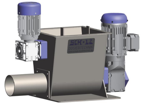
SOLO with horizontal Tube-Outlet with Agitator as optional equipment
