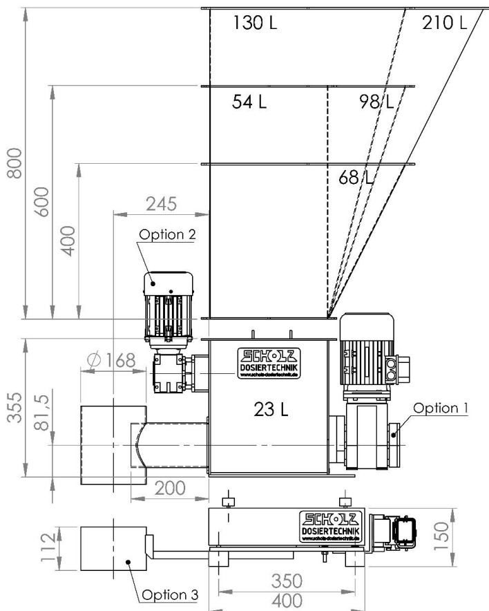
Differential-Dosierwage RATIO Loss-in-Weight-Feeder RATIO
